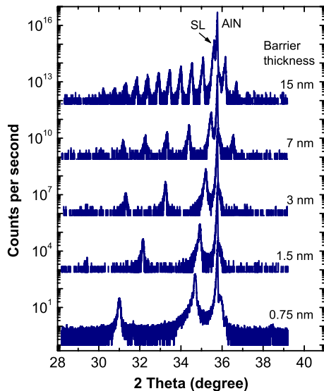
Figure 3. X-ray diffraction scans of five different superlattice periods (QW thickness 15 Å/barrier thicknesses of 7.5, 15, 30, 70, and 150 Å).
